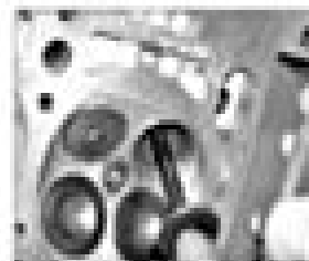
2.5a Remove the valves from the combustion chamber
