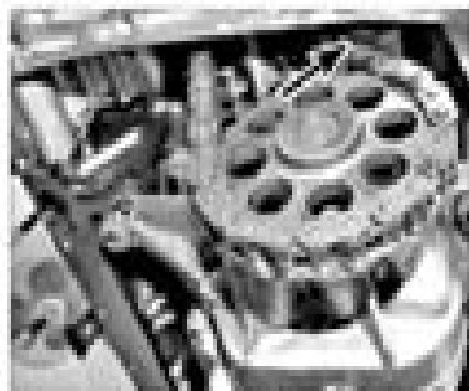
12.2 Press against the chain tensioner
